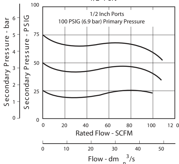
Flow Characteristics 1/2" Port
