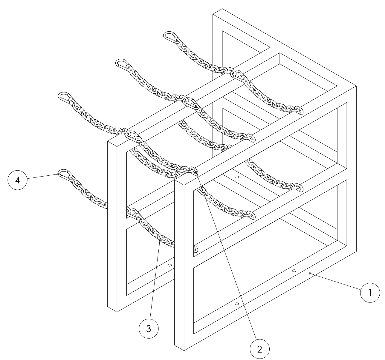
ISOMETRIC SCALE 1:8
