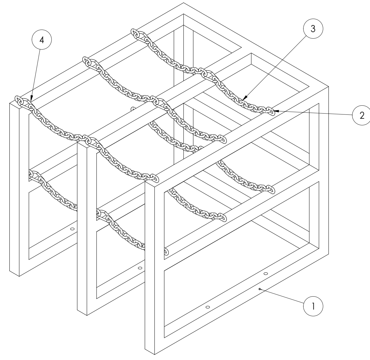
ISOMETRIC SCALE 1:8
