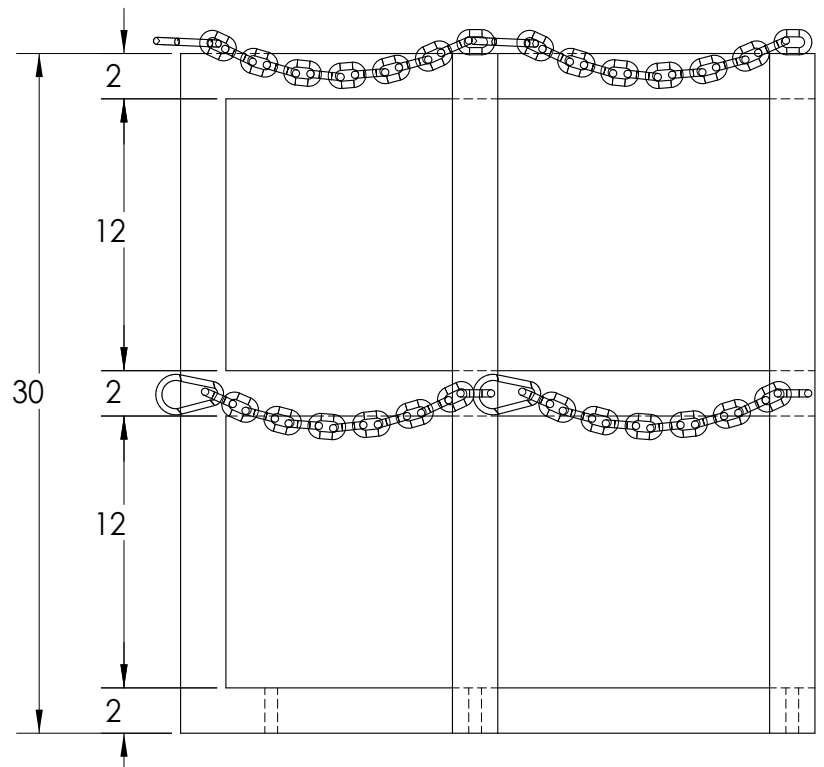
FRONT
